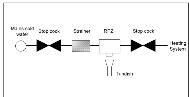
Fig. 5 Requirements Fluid Category 4 systems
