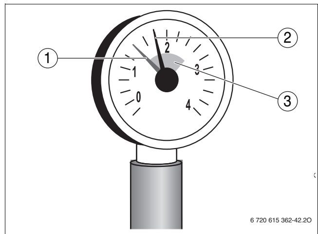
Fig. 3 Pressure gauge for open systems
