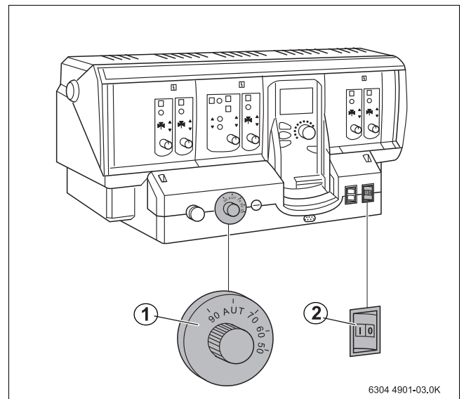
Fig. 6 Switching on the heating system
