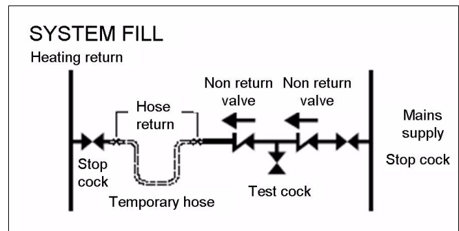
Fig. 4 Requirements Fluid Category 3 systems
